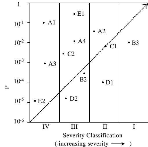
Figure 11 Criticality matrix for prioritizing failures (adapted from Bowles, 1998)
