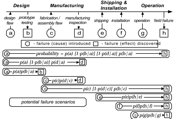
Figure 4 Failure scenarios in a product’s life cycle
