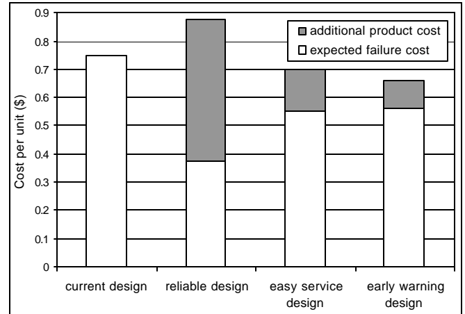
Figure 12 Life cycle cost comparison of design alternatives
