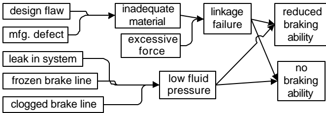
Figure 3 Scenario map for brake failures
