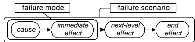
Figure 2 Failure modes and scenarios
